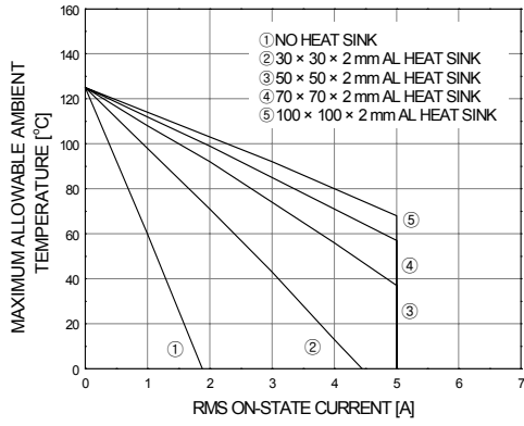
Figure 7. Allowable Ambient Temperature vs Rms On-state Current
