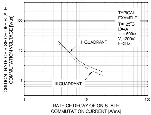
Figure 16. Commutation Characteristics
