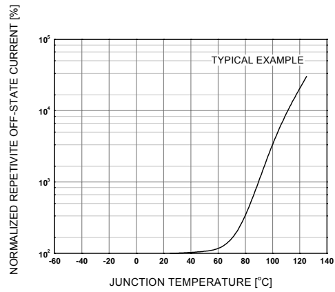
Figure 10. Repetitive Peak Off-state Current vs Junction Temperature
