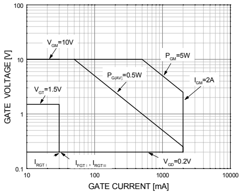
Figure 3. Gate Characteristics
