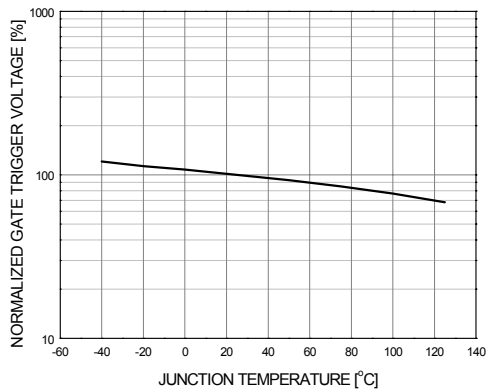
Figure 5. Gate Trigger Voltage vs Tj
