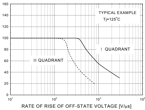
Figure 15. Breakover Voltage vs. Rate of Rise of Off-State Voltage
