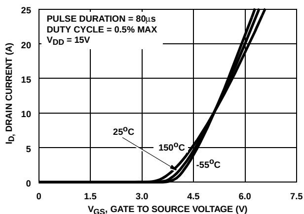
FIGURE 8. TRANSFER CHARACTERISTICS
