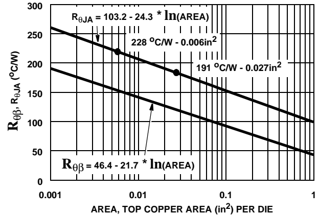
FIGURE 23. THERMAL RESISTANCE vs. MOUNTING PAD AREA
