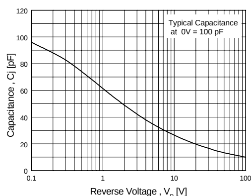
Figure 6. Typical Junction Capacitance (Damper Diode)
