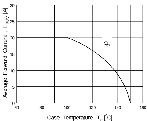
Figure 11. Forward Current Derating Curve (Modulation Diode)
