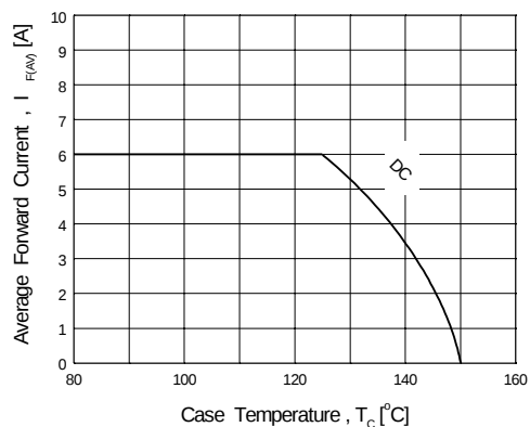
Figure 10. Forward Current Derating Curve (Damper Diode)
