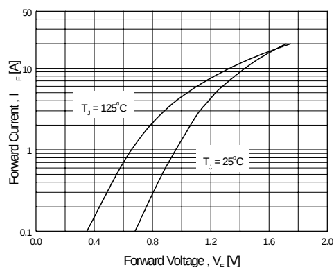
Figure 2. Typical Forward Characteristics (Damper Diode)
