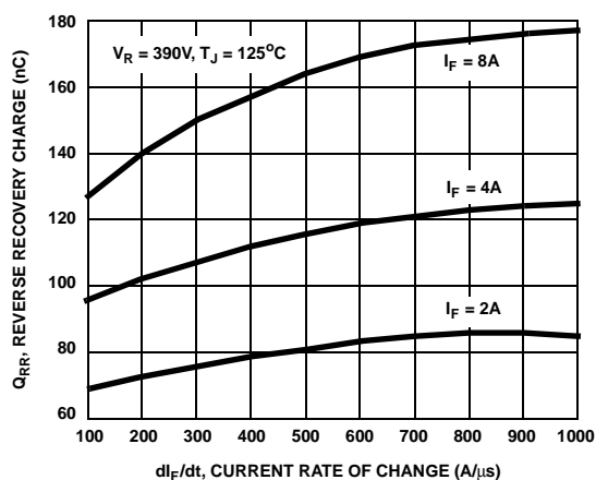
Figure 8. Reverse Recovery Charge vs dI_F/dt
