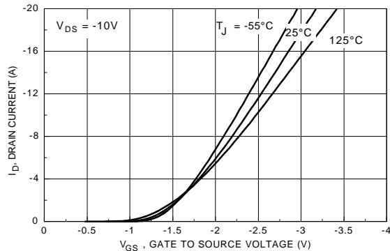
Figure 5. Transfer Characteristics.
