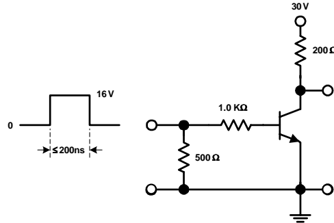
Figure 1. Saturated Turn-On Switching Time
