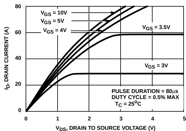
FIGURE 8. SATURATION CHARACTERISTICS
