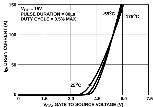
FIGURE 8. TRANSFER CHARACTERISTICS
