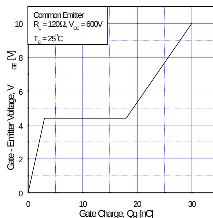
Fig 8. Typical Gate Charge Characteristic
