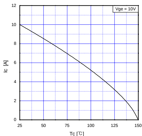
Fig 3. Maximum Collector Current vs. Case Temperature
