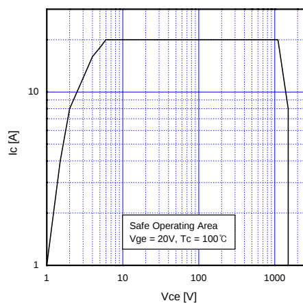
Fig 12. Turn-Off SOA
