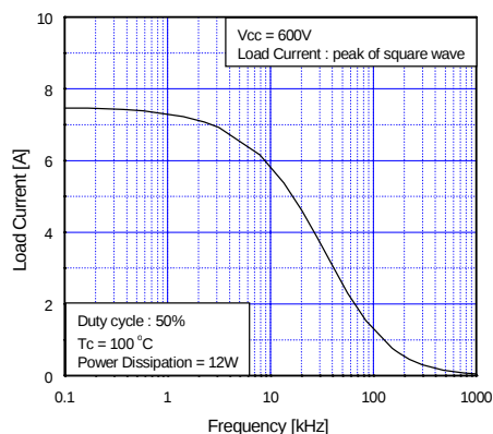
Fig 5. Load Current vs. Frequency
