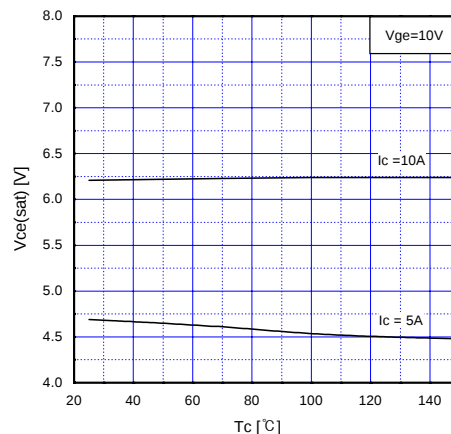
Fig 4. Saturation Voltage vs. Case Temperature
