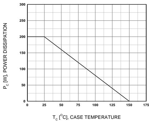
Figure 11. Power Derating
