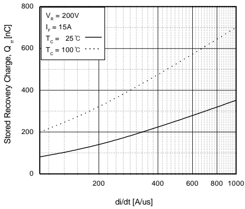
Fig 20. Stored Charge
