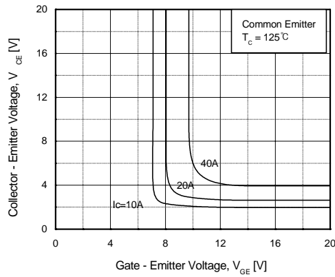
Fig 6. Saturation Voltage vs. V GE
