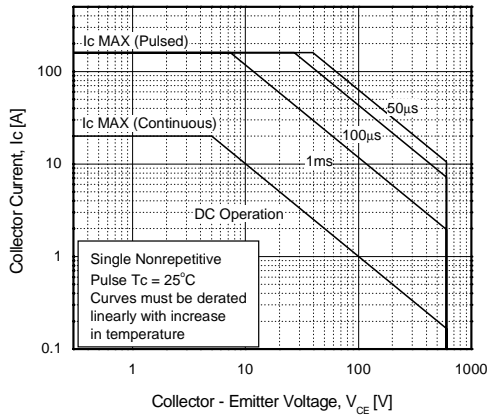
Fig 15. SOA Characteristics
