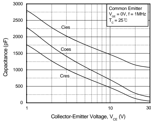
Fig 7. Capacitance Characteristics
