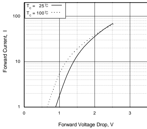
Fig 18. Forward Characteristics
