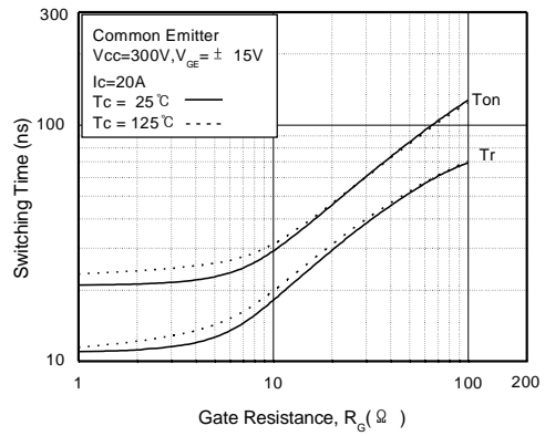
Fig 8. Turn-On Characteristics vs. Gate Resistance
