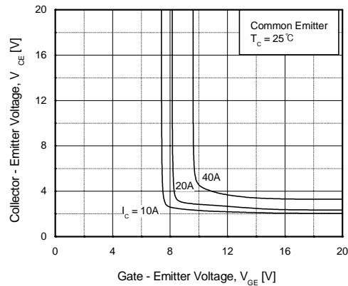
Fig 5. Saturation Voltage vs. V GE
