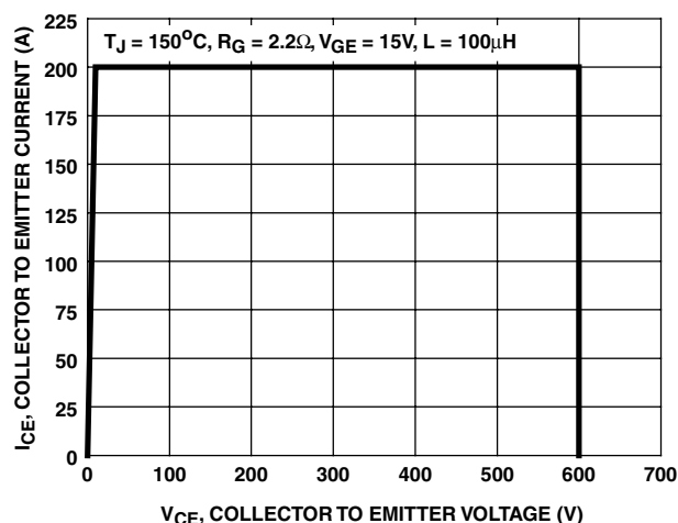
FIGURE 2. MINIMUM SWITCHING SAFE OPERATING AREA
