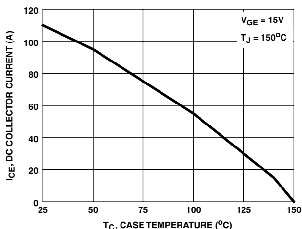
FIGURE 1. DC COLLECTOR CURRENT vs CASE TEMPERATURE
