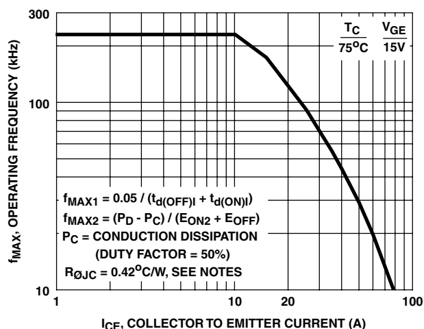
FIGURE 3. OPERATING FREQUENCY vs COLLECTOR TO EMITTER CURRENT
