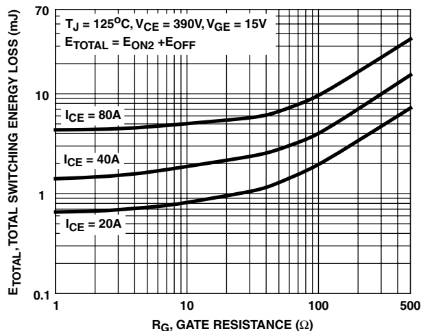
FIGURE 16. TOTAL SWITCHING LOSS vs GATE RESISTANCE
