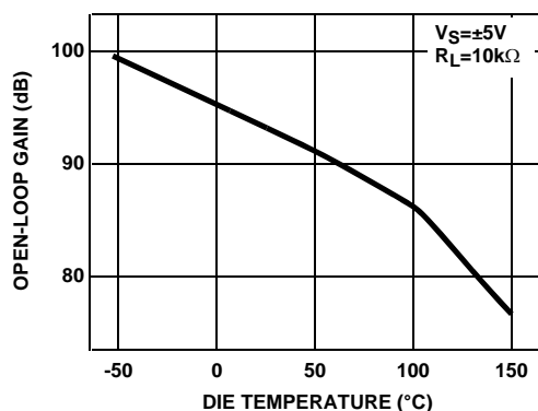
FIGURE 7. OPEN-LOOP GAIN vs TEMPERATURE
