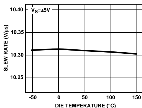
FIGURE 8. SLEW RATE vs TEMPERATURE
