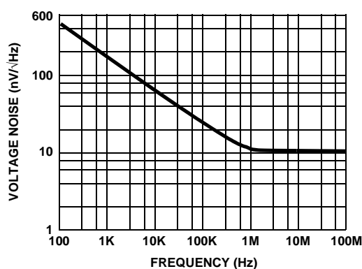
FIGURE 18. INPUT VOLTAGE NOISE SPECTRAL DENSITY vs FREQUENCY
