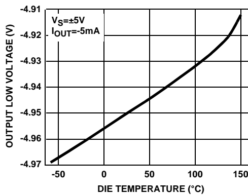
FIGURE 6. OUTPUT LOW VOLTAGE vs TEMPERATURE
