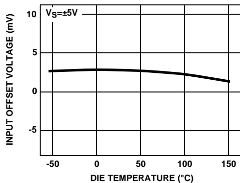
FIGURE 3. INPUT OFFSET VOLTAGE vs TEMPERATURE
