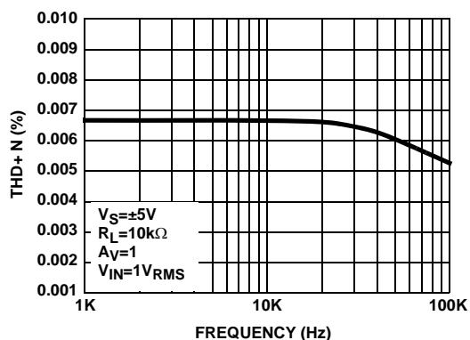
FIGURE 19. TOTAL HARMONIC DISTORTION + NOISE vs FREQUENCY
