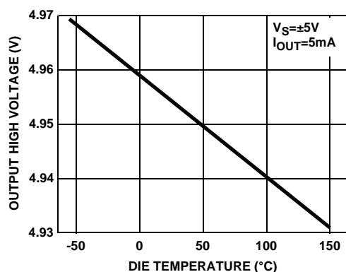
FIGURE 5. OUTPUT HIGH VOLTAGE vs TEMPERATURE
