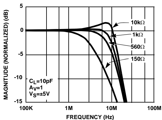
FIGURE 12. FREQUENCY RESPONSE FOR VARIOUS R_L
