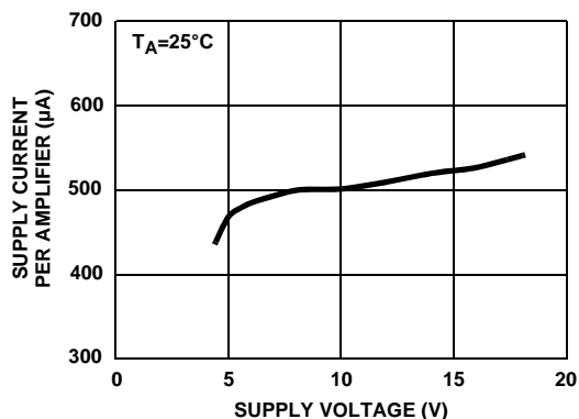
FIGURE 10. SUPPLY CURRENT PER AMPLIFIER vs SUPPLY VOLTAGE
