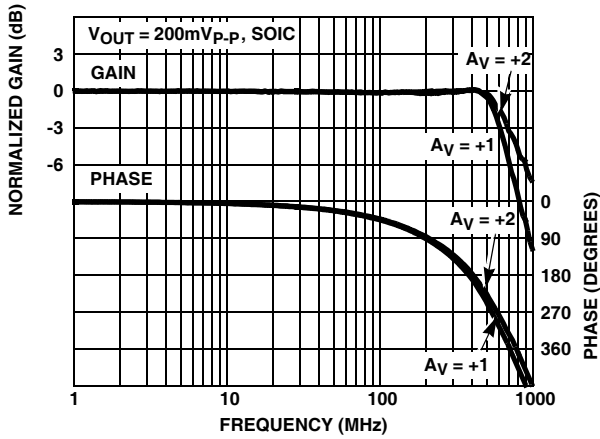
FIGURE 12. FREQUENCY RESPONSE
