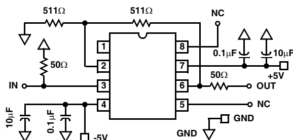
FIGURE 2. HFA11XXEVAL SCHEMATIC
