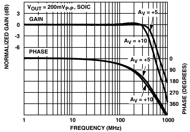
FIGURE 13. FREQUENCY RESPONSE
