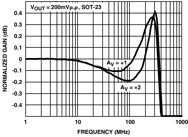
FIGURE 18. GAIN FLATNESS
