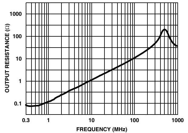
FIGURE 21. CLOSED LOOP OUTPUT RESISTANCE
