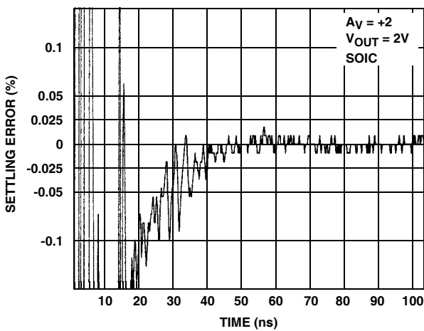
FIGURE 22. SETTLING RESPONSE
