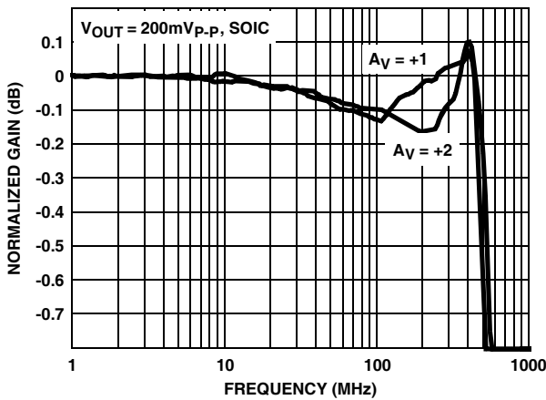
FIGURE 14. GAIN FLATNESS
