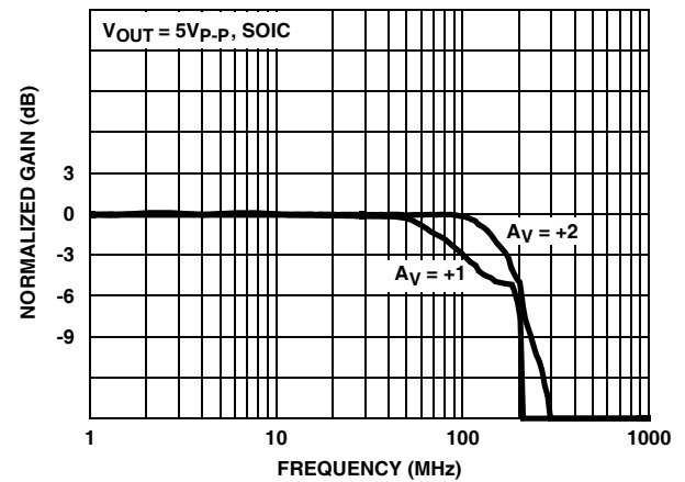
FIGURE 15. FULL POWER BANDWIDTH
