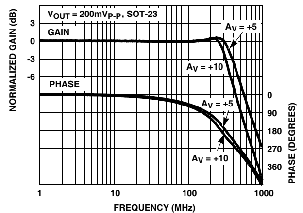
FIGURE 17. FREQUENCY RESPONSE
