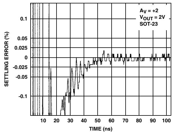
FIGURE 23. SETTLING RESPONSE
