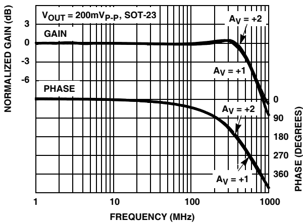
FIGURE 16. FREQUENCY RESPONSE
