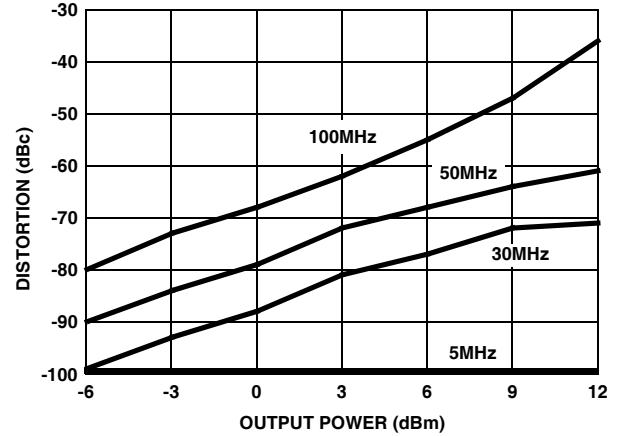
FIGURE 27. 3rd HARMONIC DISTORTION vs P OUT
