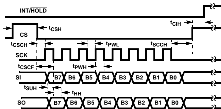
FIGURE 1. SPI TIMING
