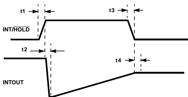
FIGURE 2. INTEGRATOR TIMING
