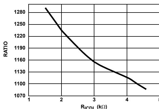
FIGURE 1. THE RATIO USED IN THE CHARGE CURRENT CALCULATION vs. R_{ICDL}
