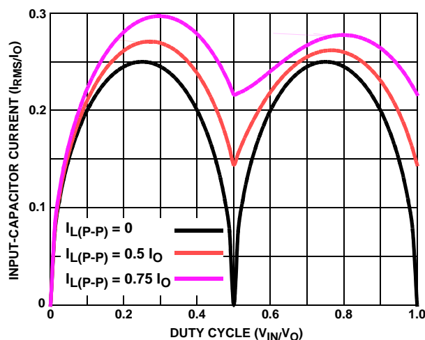
FIGURE 22. NORMALIZED INPUT-CAPACITOR RMS CURRENT FOR 2-PHASE CONVERTER
