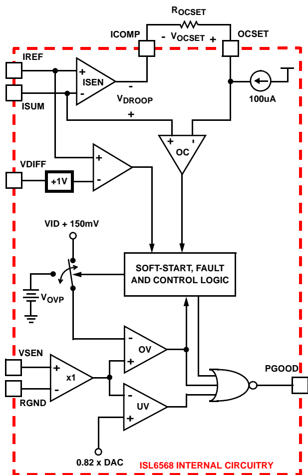
FIGURE 13. POWER GOOD AND PROTECTION CIRCUITRY
