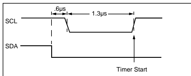
Figure 3. Watchdog Restart
