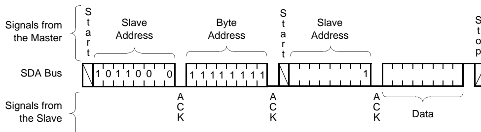
Figure 9. Read Sequence
