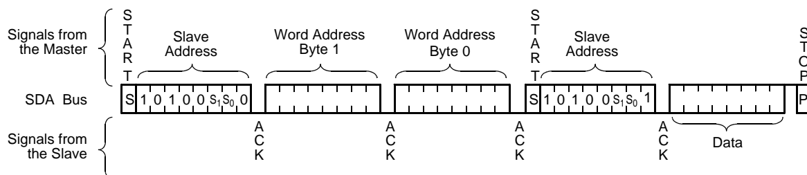
Figure 13. Random Address Read Sequence
