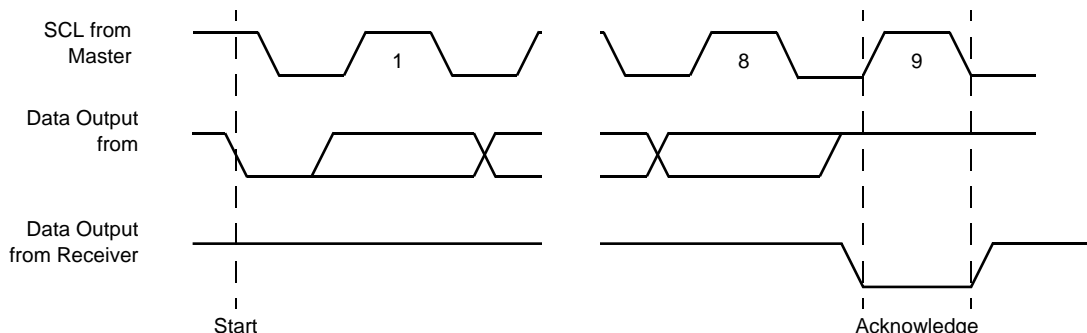
Figure 7. Acknowledge Response From Receiver
