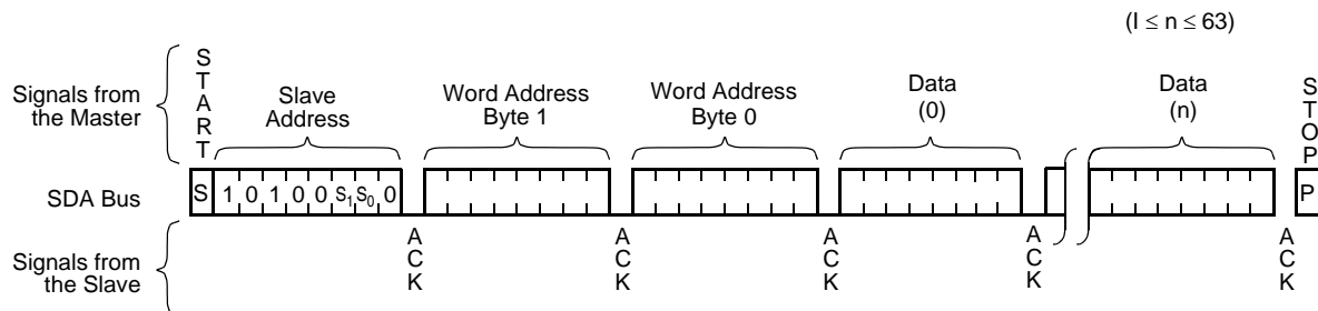
Figure 9. Page Write Operation
