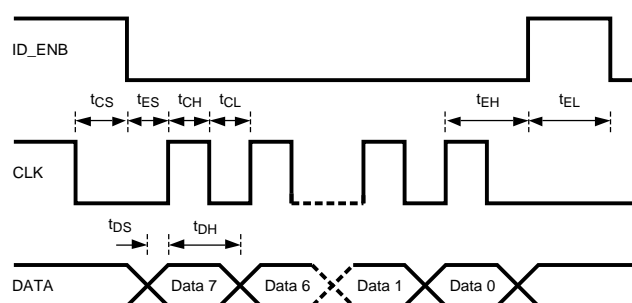
Figure 65. SPI Timing Diagram
