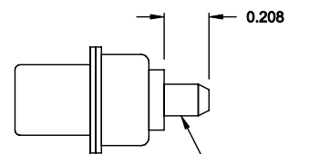
POWER CONTACTS
