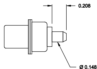
POWER CONTACTS
