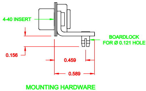
MOUNTING HARDWARE
