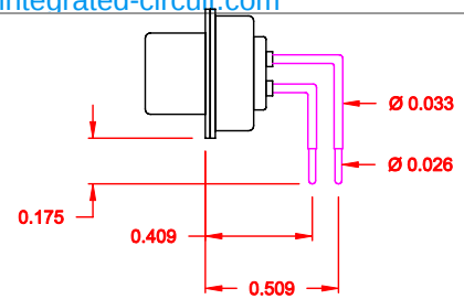
SIGNAL CONTACTS
