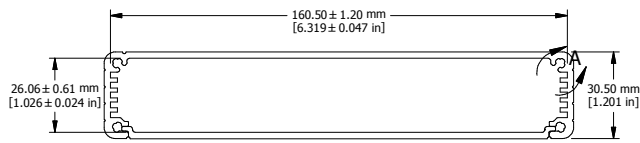
EXTRUSION
