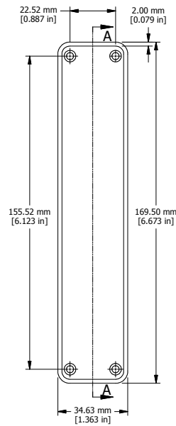
CLOSED BEZEL
