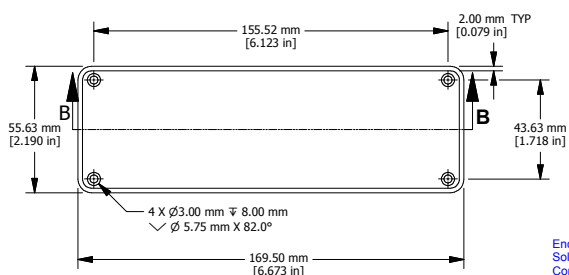
EXTRUSION DESIGNED FOR 160MM WIDE PC BOARD
