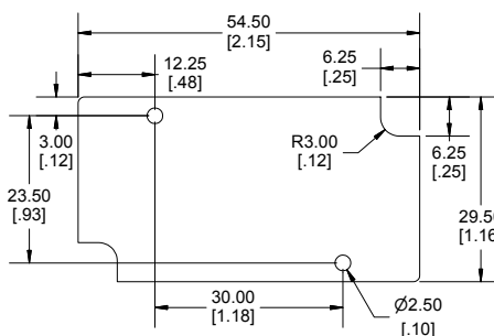
MAXIMUM P.C. BOARD SIZE
