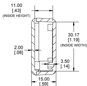
END VIEW SECTION B-B
