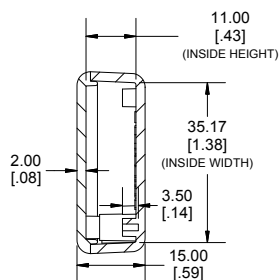
END VIEW SECTION B-B
