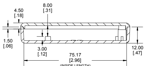
SIDE VIEW SECTION A-A
