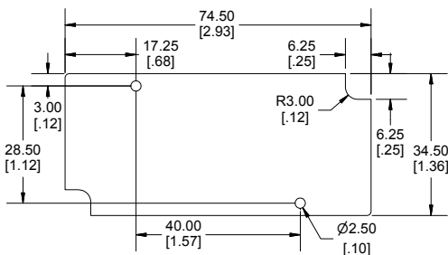
MAXIMUM P.C. BOARD SIZE
