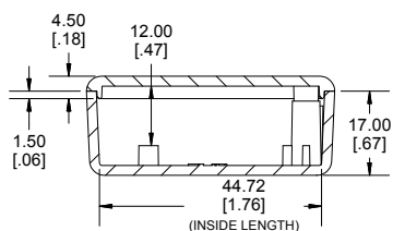
SIDE VIEW SECTION A-A
