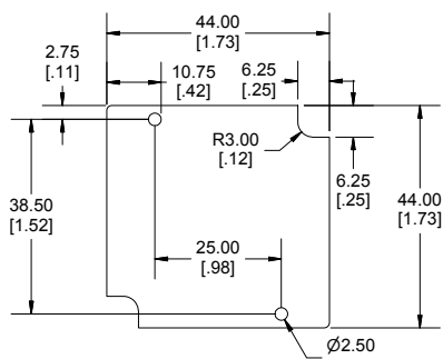
MAXIMUM P.C. BOARD SIZE
