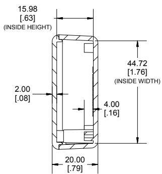
END VIEW SECTION B-B
