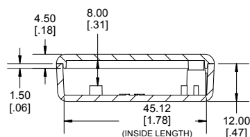
SIDE VIEW SECTION A-A
