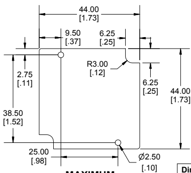
MAXIMUM P.C. BOARD SIZE
