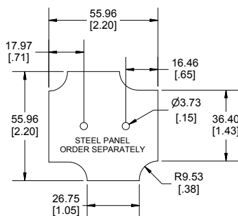
SECTION B-B END VIEW
