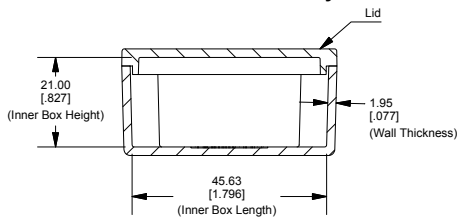
SECTION B-B Side View of Assembly
