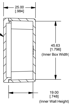
Top View Looking Inside Box
