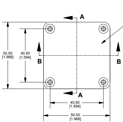
Top View of Assembly
