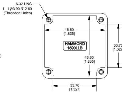
Top View Looking Inside Box
