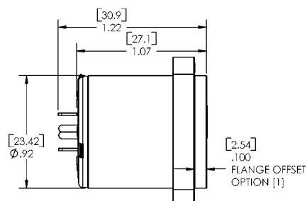
[PC] TERMINALS
