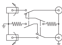
NON-NORMALLED TERMINATED
