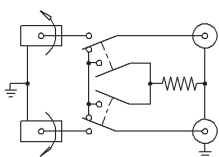
NORMALLED TERMINATED
