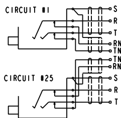
NORMALS OUT
