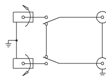
NORMALLED NON-TERMINATED
