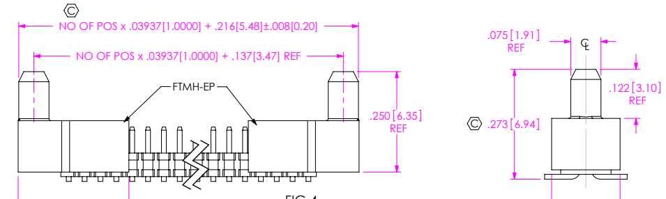
FIG 4 -EP: GUIDE POST FTMH-125-03-X-DV-EP SHOWN (DIFFERENT AS SHOWN, OTHERWISE SAME AS FIG 1)
