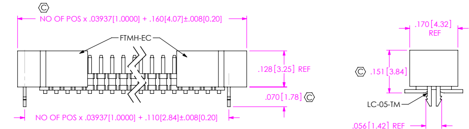
FIG 5 -EC: LOCKING CLIP FTMH-125-03-X-DV-EC SHOWN (DIFFERENT AS SHOWN, OTHERWISE SAME AS FIG 1)
