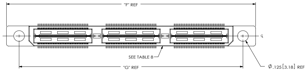
FIG 8 (QTH-090-01-X-D-GP SHOWN) (SAME AS FIG 1, EXCEPT AS SHOWN) (AVAILABLE ON -01 & -02 ONLY)
