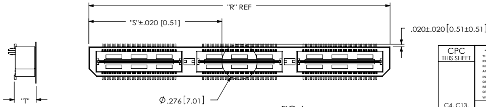
FIG 4 -K: POLYIMIDE FILM PAD OPTION (USE K-DOT-.276-.375-.005)
