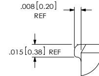
DETAIL 'E' SCALE 12:1
