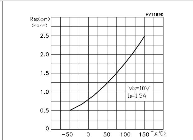
Figure 14. Normalized on resistance vs temperature
