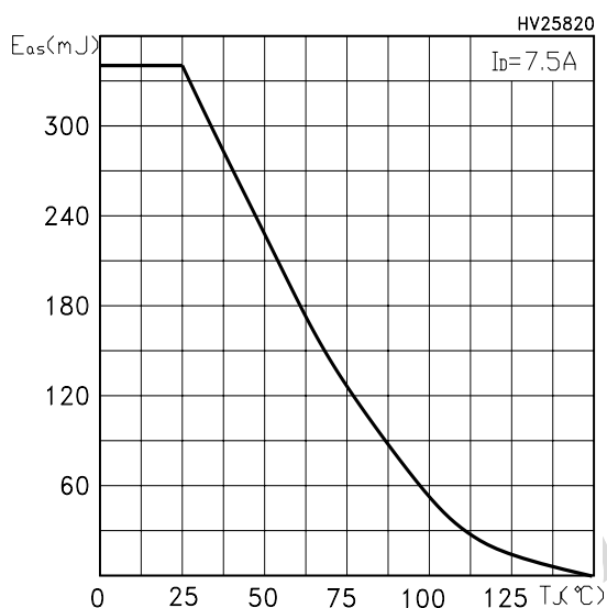
Figure 16: Avalanche Energy vs Temperature
