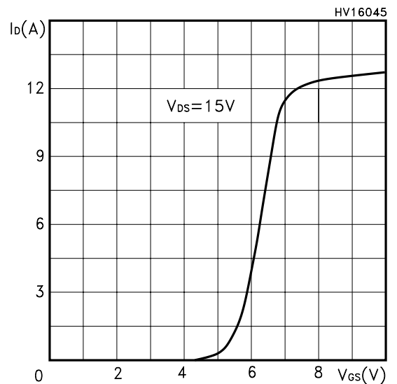
Figure 8: Transfer Characteristics
