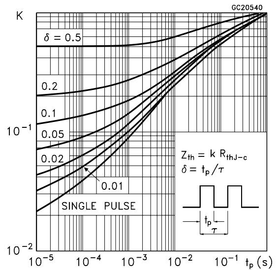
Figure 7: Thermal Impedance for TO-220FP
