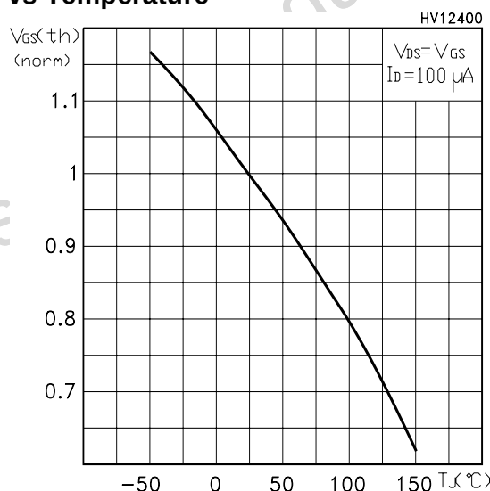
Figure 11: Normalized Gate Threshold Voltage vs Temperature
