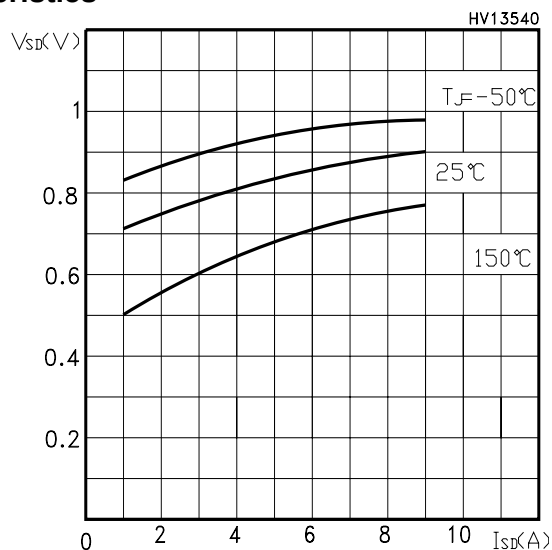
Figure 17: Source-Drain Diode Forward Characteristics
