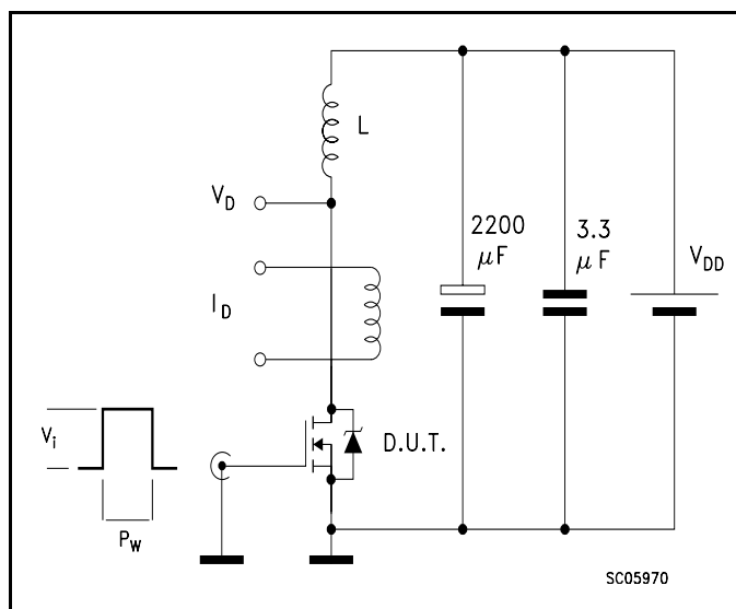
Figure 19: Switching Times Test Circuit For Resistive Load
