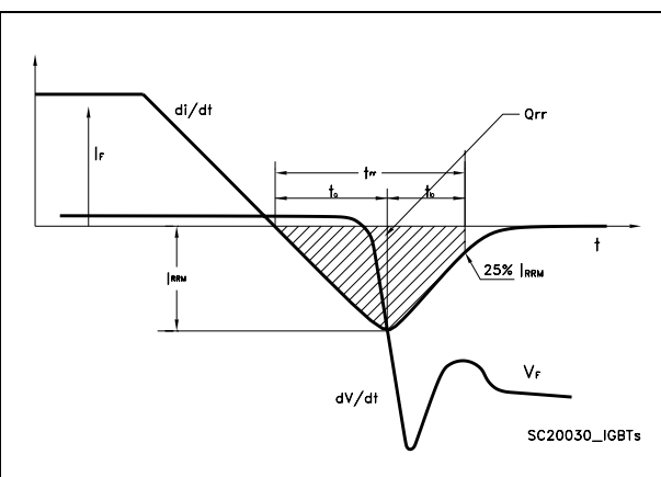
Figure 21. Diode recovery time waveform
