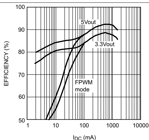
Figure 9. Efficiency vs Load Current (330 kHz)
