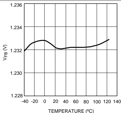
Figure 1. VFB vs Temperature
