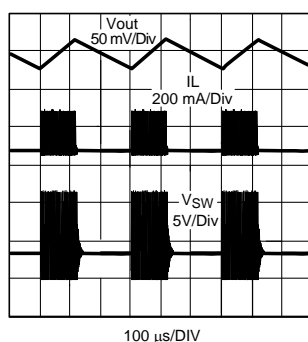
Figure 15. Sleep Mode Waveforms 25-mA Load, Vin = 12 V
