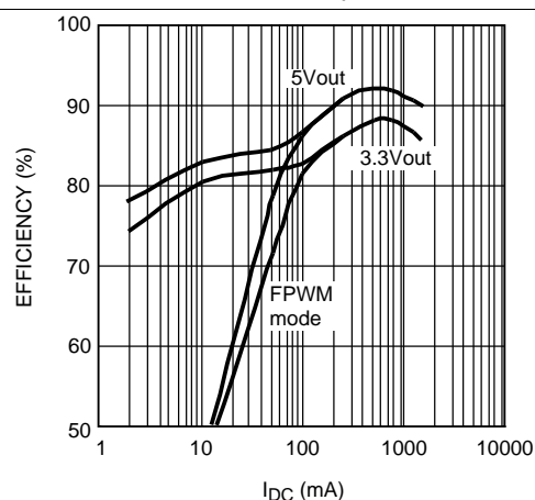
Figure 10. Efficiency vs Load Current (500 kHz)
