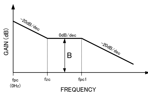
Figure 22. Feedback Transfer Function
