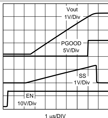
Figure 11. Startup Waveforms
