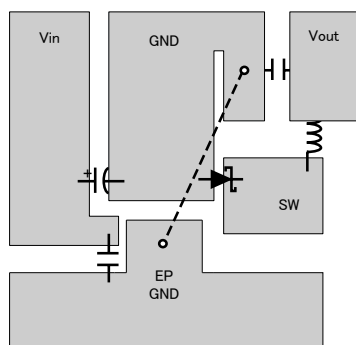
Figure 26. Example PCB Layout
