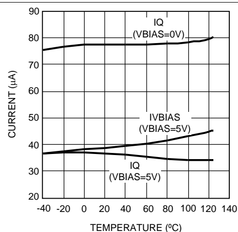
Figure 3. I_Q and I_{VBIAS} vs Temperature (Sleep Mode)
