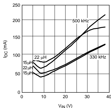
Figure 16. Sleep Mode Threshold vs Vin Vout = 3.3 V
