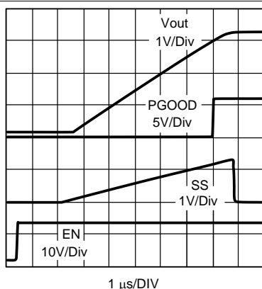
Figure 24. Startup Waveforms
