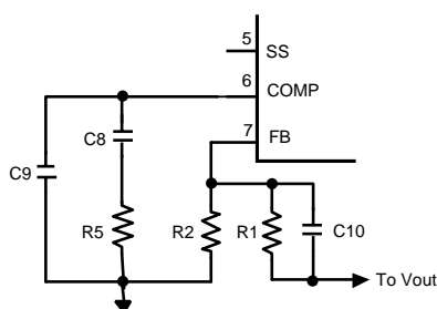
Figure 23. Compensation Network
