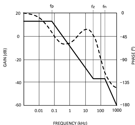
Figure 21. Control-Output Transfer Function
