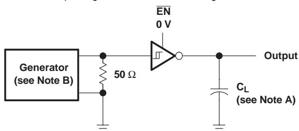
TEST CIRCUIT
