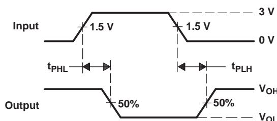
VOLTAGE WAVEFORMS
