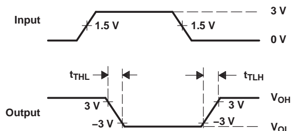
VOLTAGE WAVEFORMS
