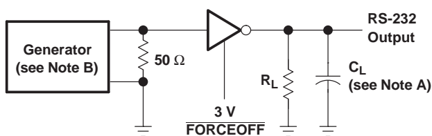
TEST CIRCUIT
