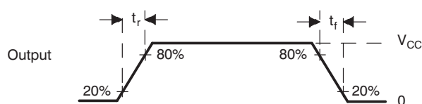
Figure 10. CMOS-Level Outputs
