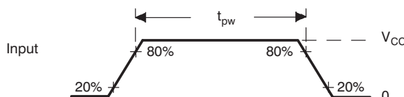
Figure 11. CMOS-Level Inputs
