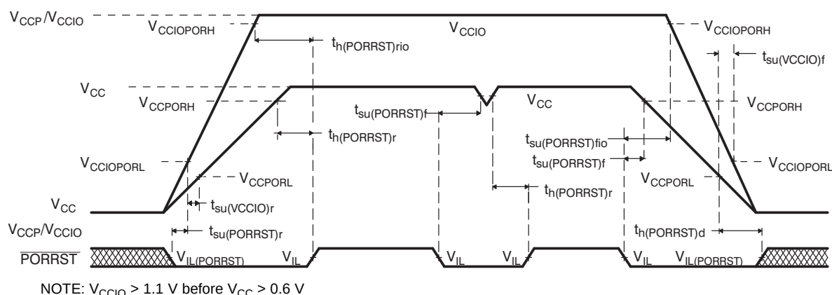
Figure 8. \overline{PORRST} Timing Diagram
