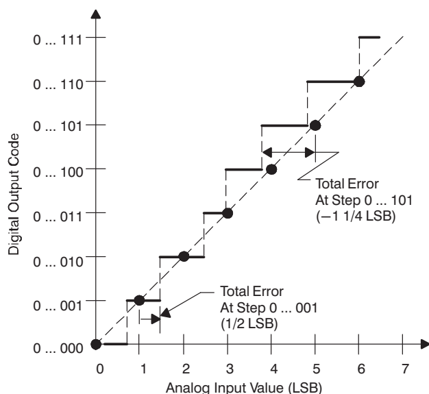
Figure 21. Absolute Accuracy (Total) Error
