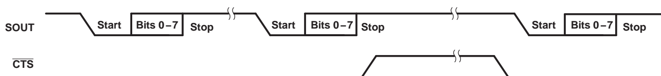
Figure 2. \overline{\text{CTS}} Functional Timing Waveforms
