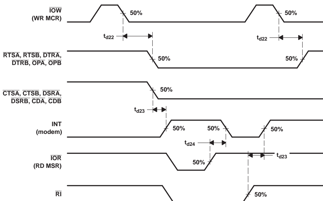
Figure 21. Modem Control Timing Waveforms
