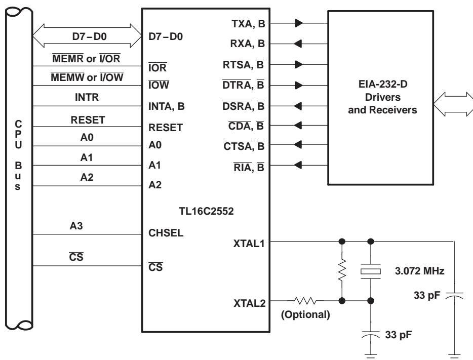
Figure 25. Basic TL16C2552 Configuration
