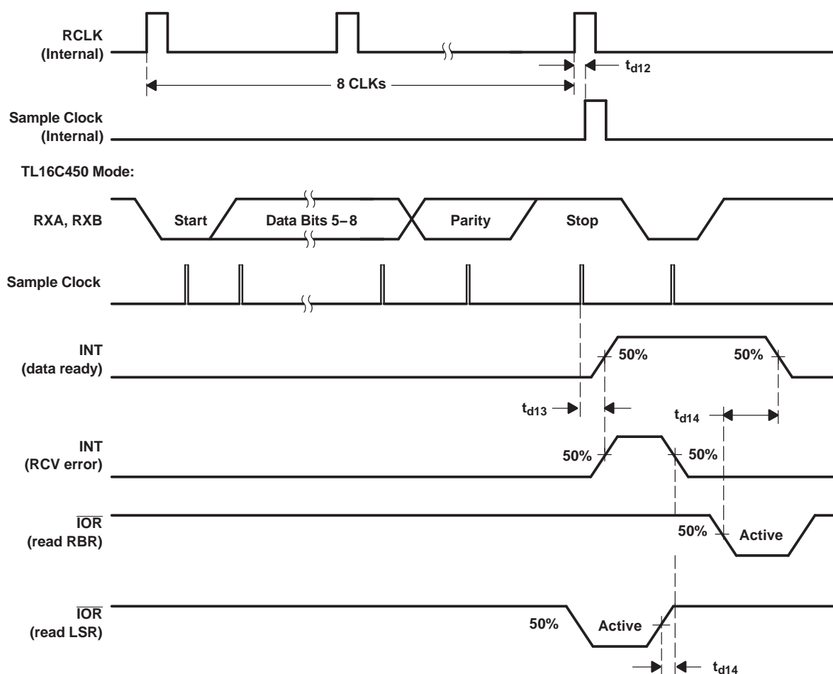
Figure 13. Receiver Timing Waveforms
