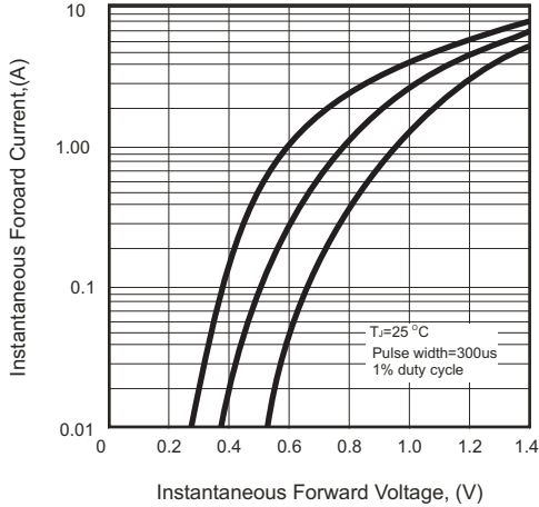
Fig.3 - Forward Characteristics
