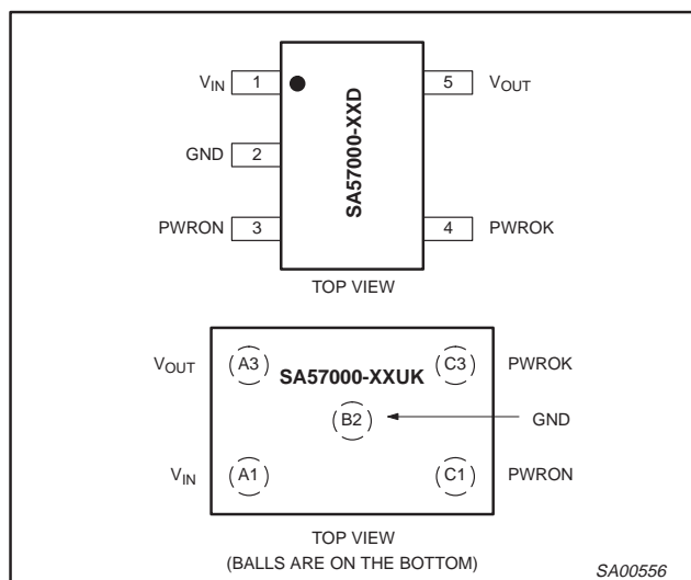
Figure 2. Pin configurations.
