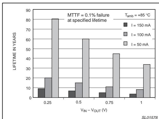
Figure 12. Lifetime versus V_{IN} - V_{OUT} for 3 output currents.
