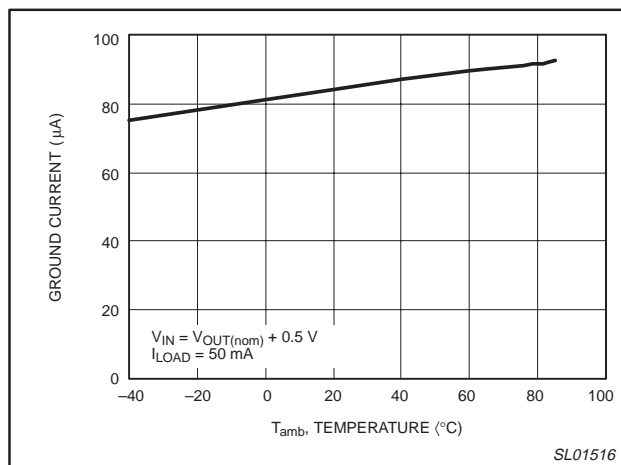
Figure 4. Ground current versus temperature.
