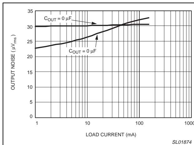
Figure 10. Output noise versus load current.
