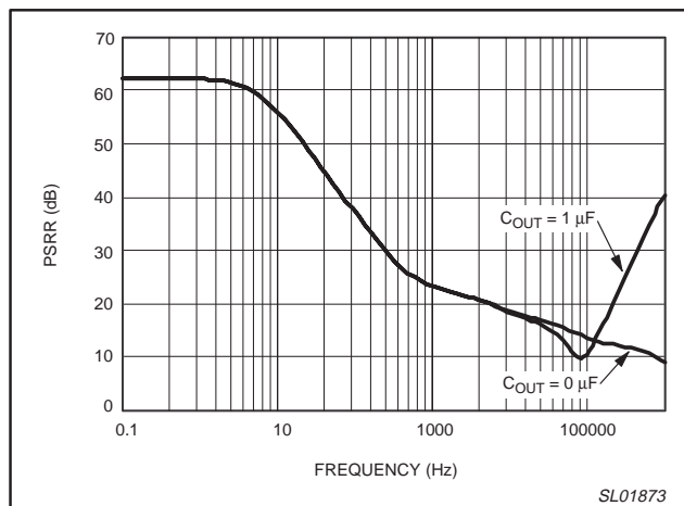
Figure 9. Power supply rejection ratio versus frequency.
