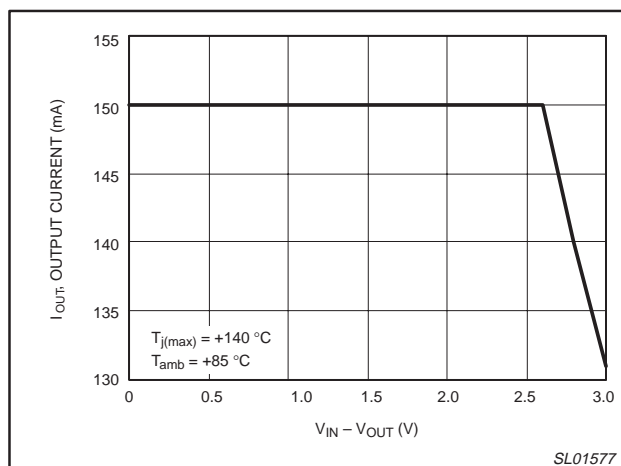
Figure 8. Maximum I_{OUT} versus V_{IN} - V_{OUT} .
