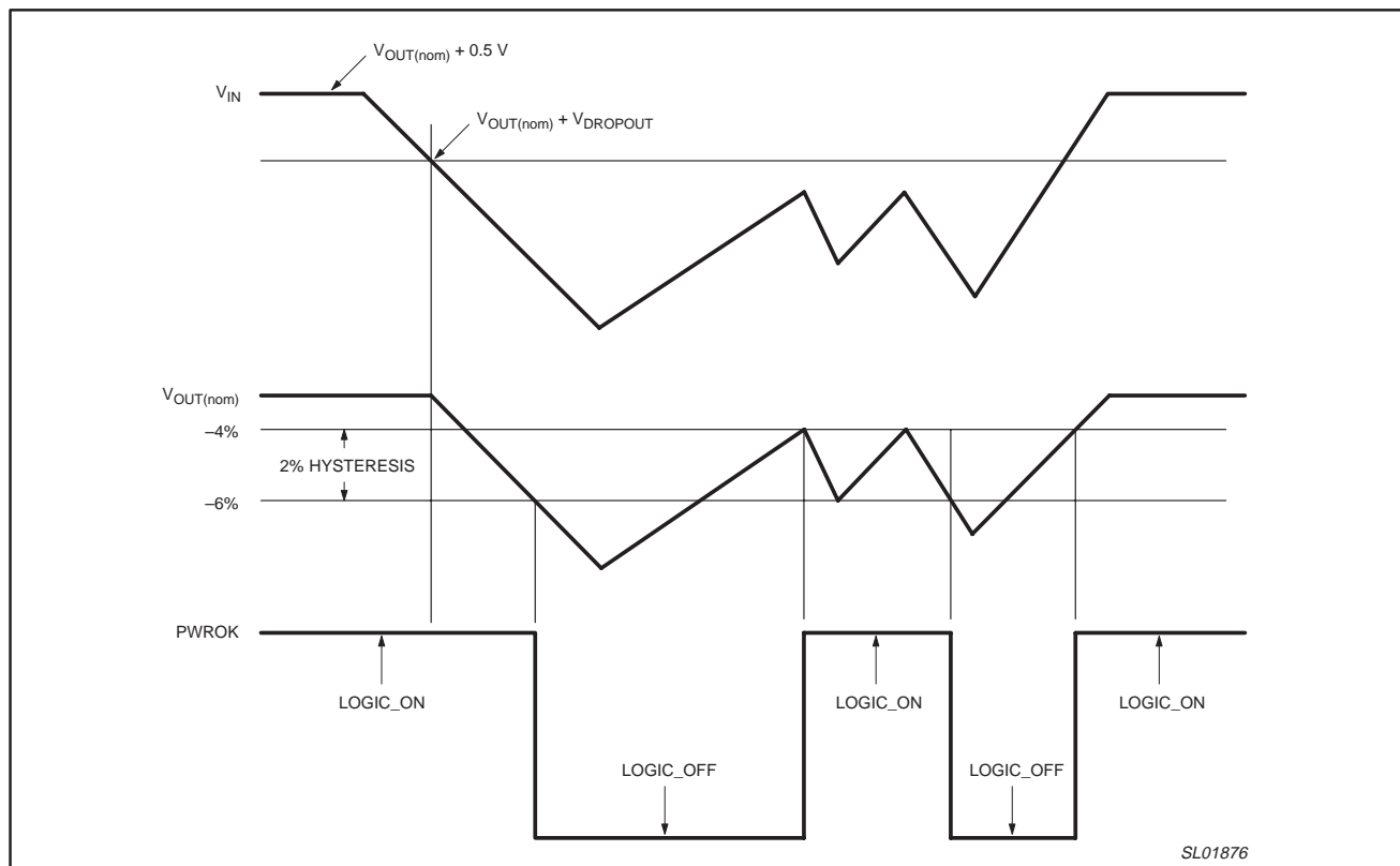
Figure 13. Timing diagram.
