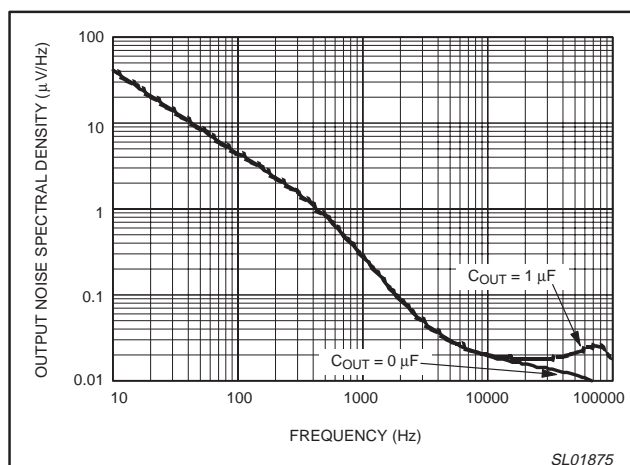
Figure 11. Output noise spectral density versus frequency.
