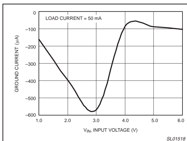
Figure 6. Ground current versus input voltage with load.
