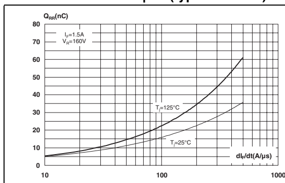
Figure 9. Reverse recovery charges versus di_F/dt (typical values)
