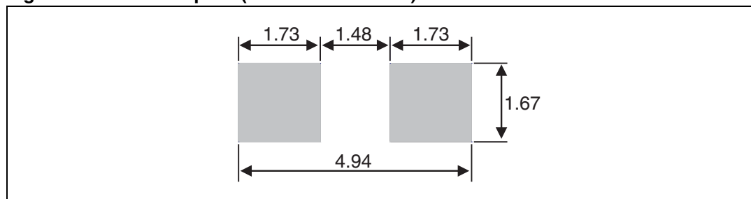
Figure 17. SMA footprint (dimensions in mm)
