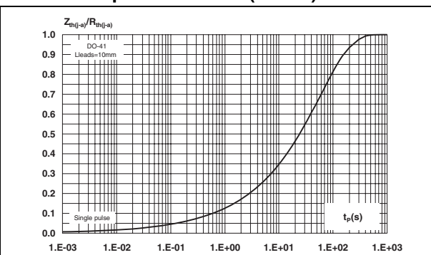
Figure 6. Relative variation of thermal impedance junction to case versus pulse duration (DO-41)
