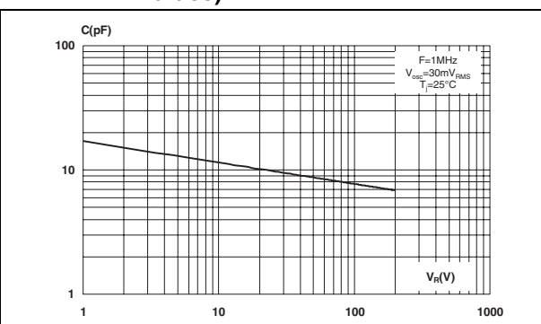
Figure 8. Junction capacitance versus reverse applied voltage (typical values)
