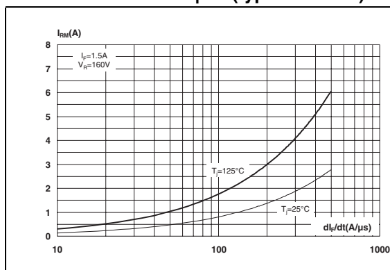
Figure 11. Peak reverse recovery current versus di_F/dt (typical values)
