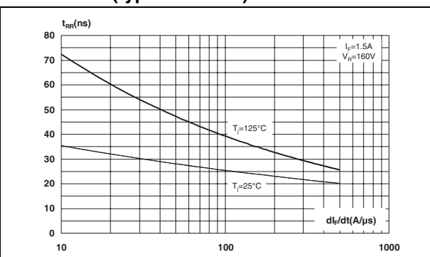
Figure 10. Reverse recovery time versus di_F/dt (typical values)
