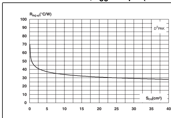
Figure 11. Thermal resistance, junction to ambient, versus copper surface under tab - Epoxy printed circuit board FR4, e_{CU} = 35 \mu m (D 2 PAK )
