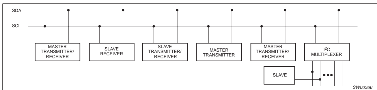
Figure 7. System configuration
