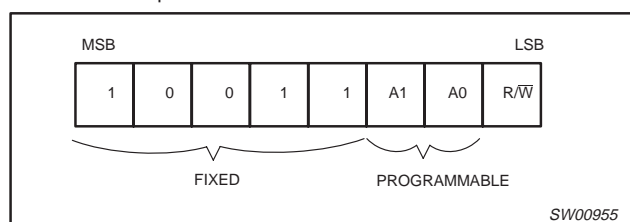
Figure 3. Slave address
