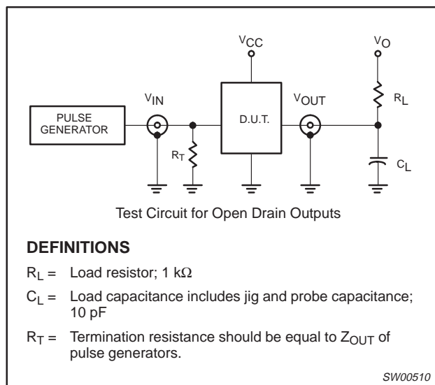
Figure 14. Test circuit
