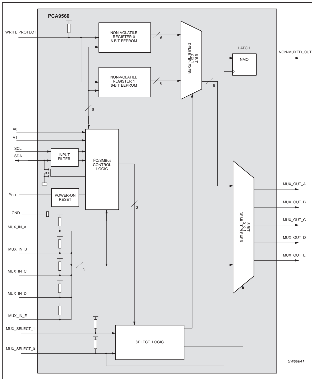
Figure 2. Block diagram
