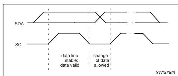
Figure 5. Bit transfer
