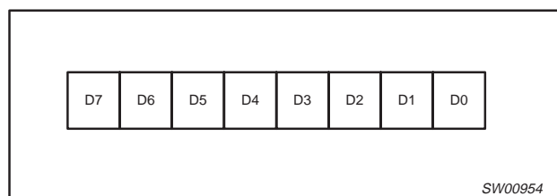
Figure 4. Control Register
