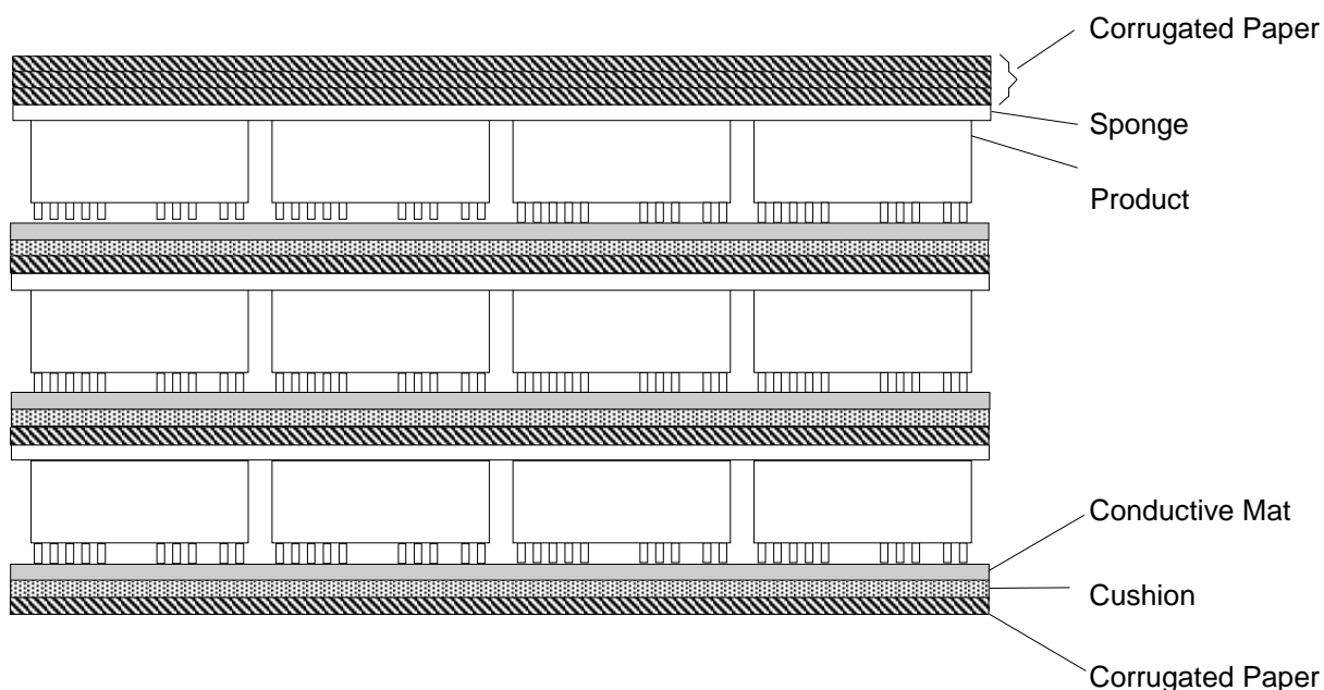
Fig1-2.Side View
