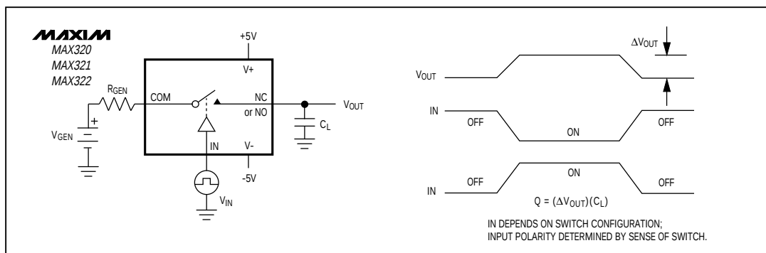
Figure 4. Charge Injection
