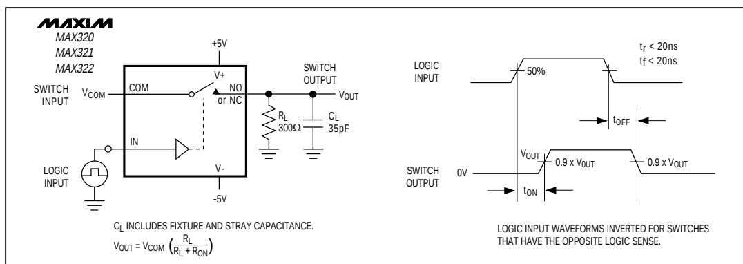
Figure 2. Switching Time
