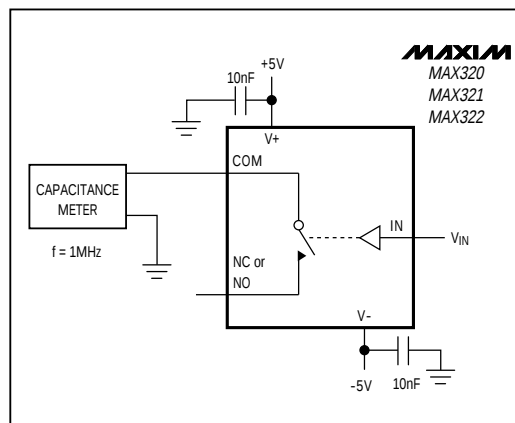
Figure 8. Channel-On Capacitance
