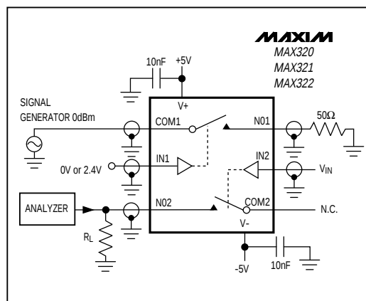
Figure 6. Crosstalk
