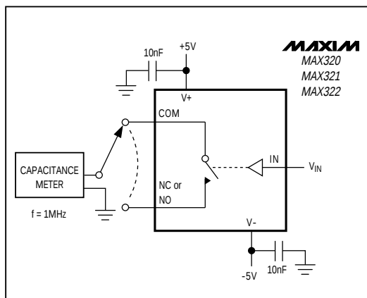
Figure 7. Channel-Off Capacitance
