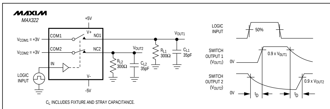
Figure 3. Break-Before-Make Interval (MAX322 only)
